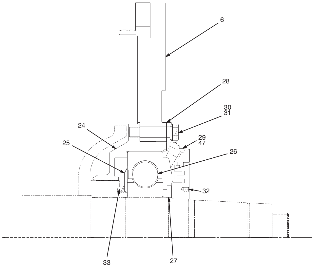
DETAIL C
