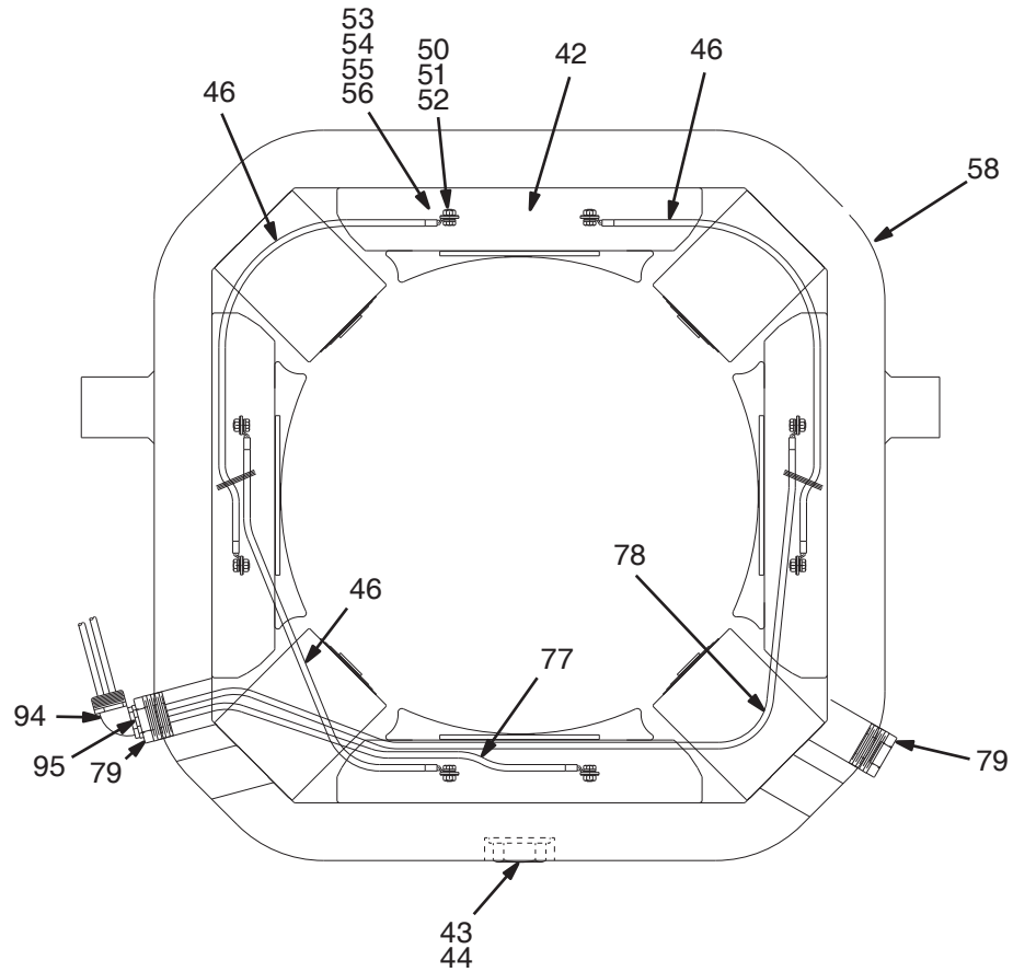
VIEW OF PINION END
