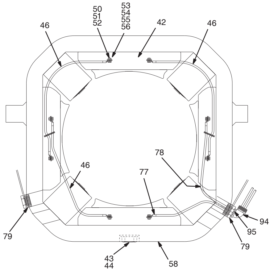
VIEW OF PINION END
