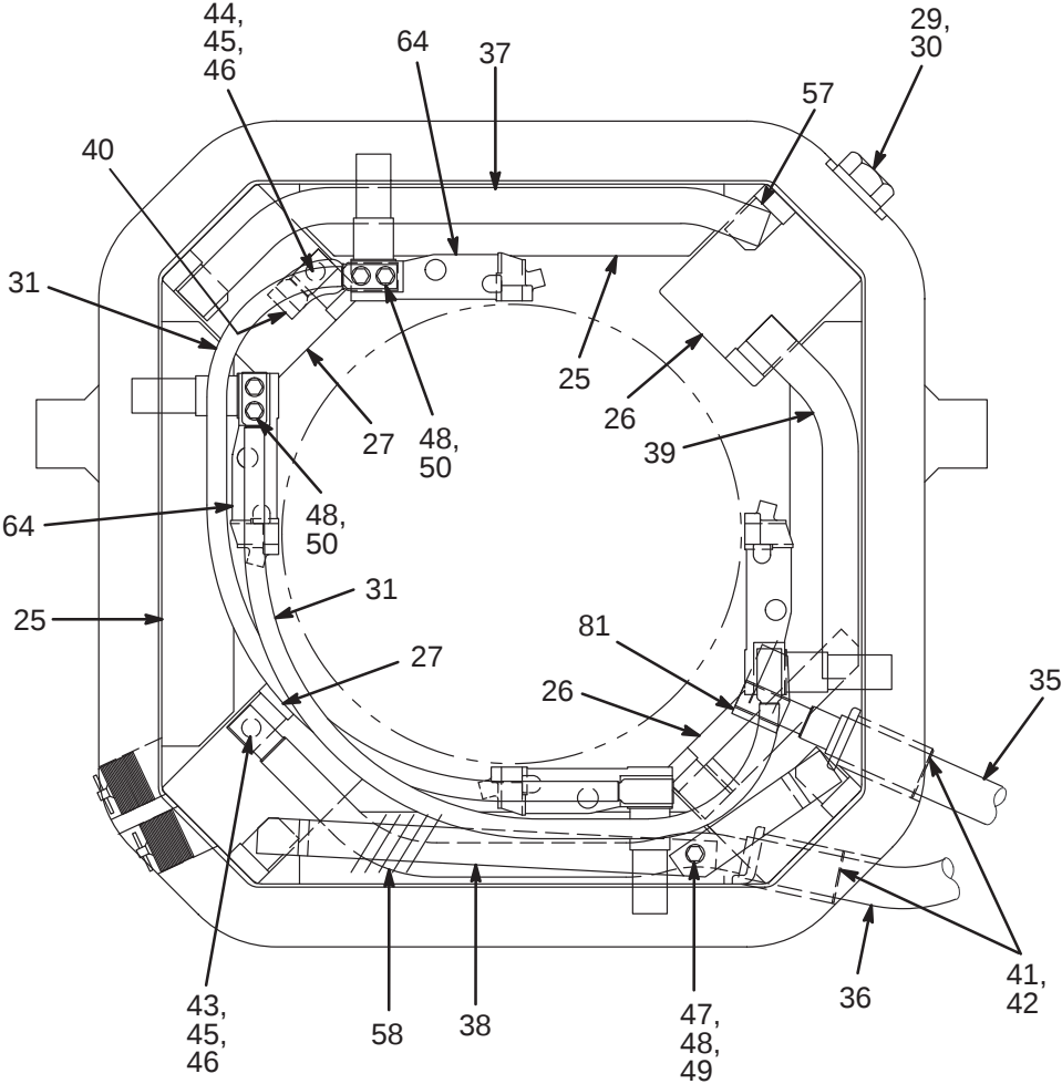
VIEW OF COMM. END
