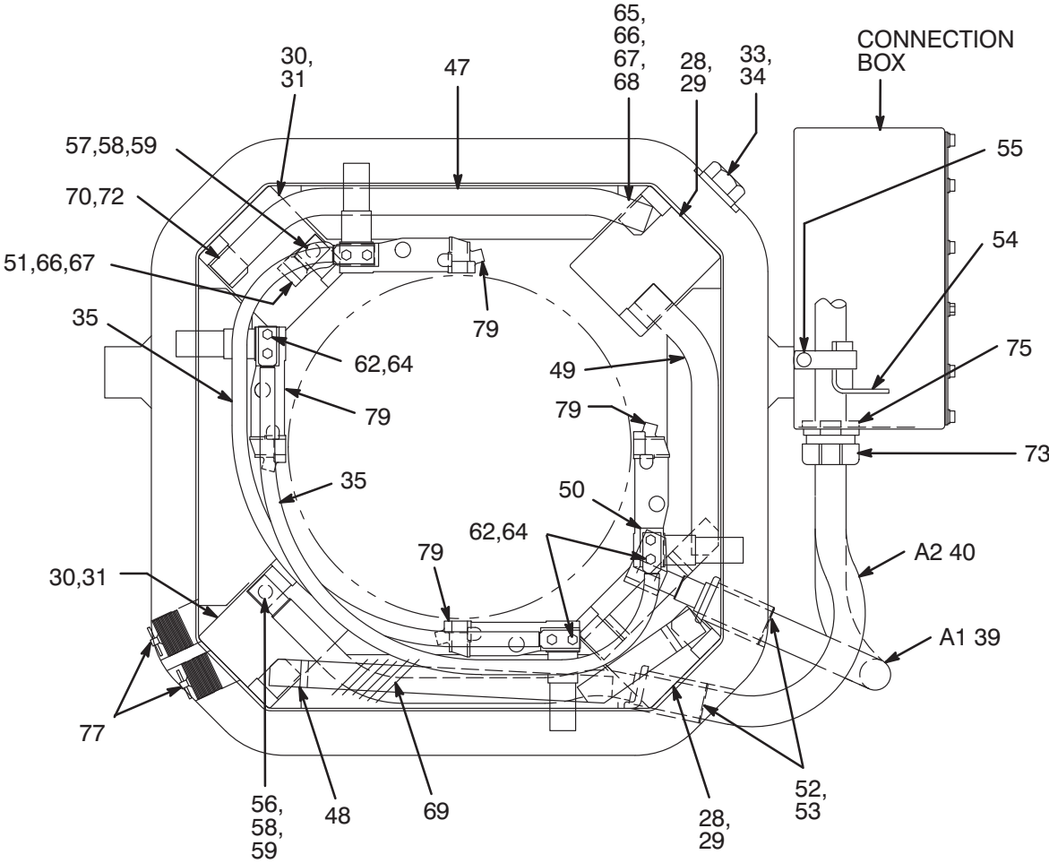
VIEW OF COMMUTATOR END
